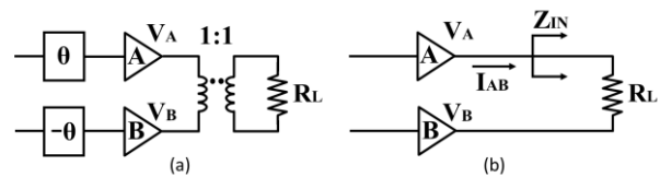
Fig. 5. (a) HRPAs transformer output power combiner, (b) simplified model of power combiner loading on the drivers.
